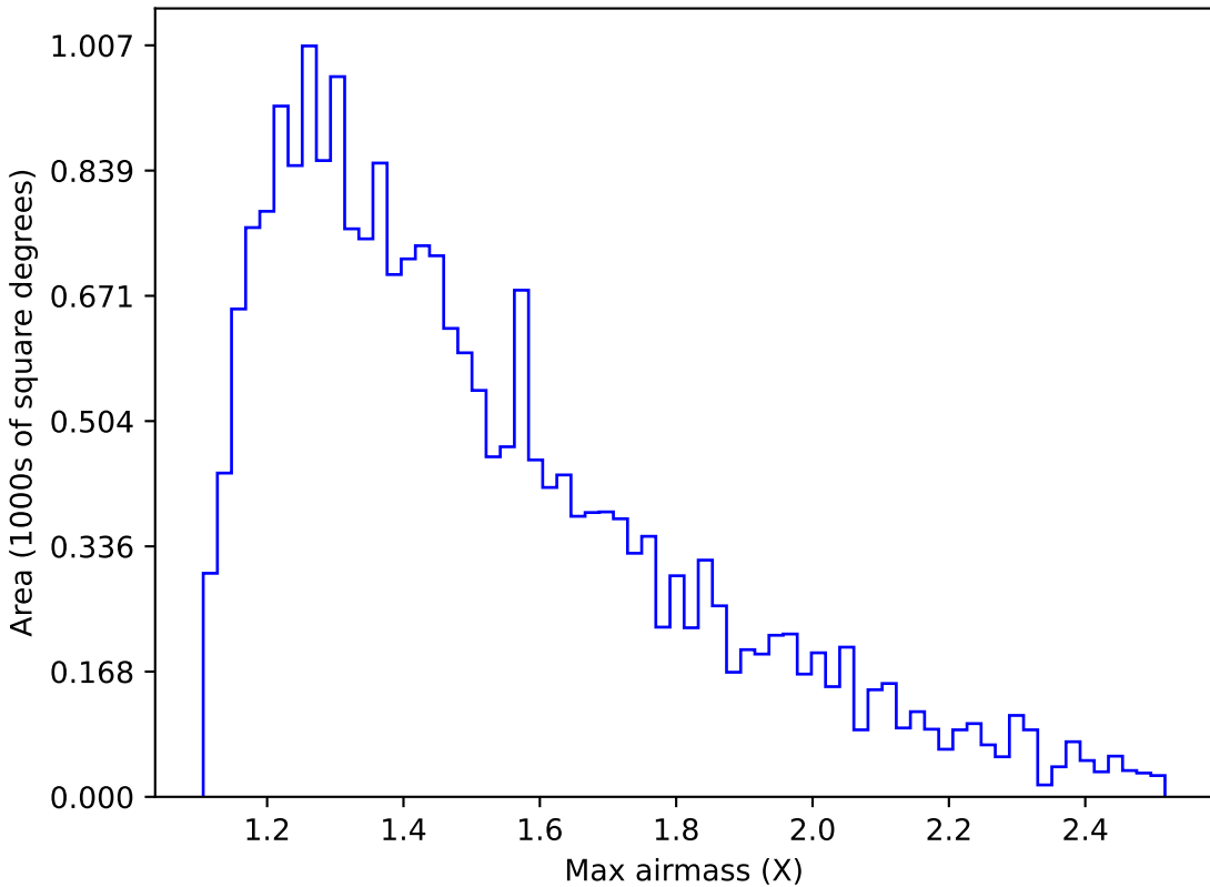
all_long_v3.4_10yrs Yr 1 u band: Max airmass
