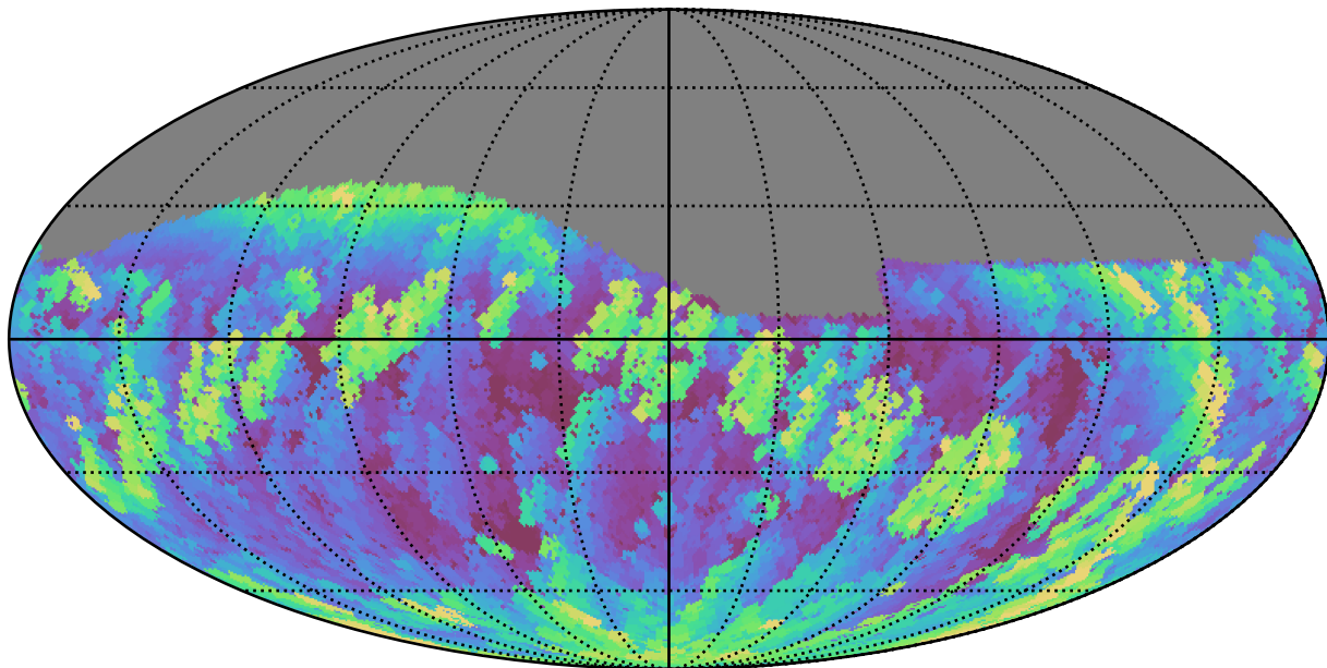
all_long_v3.4_10yrs Yr 1 r band: Max airmass
