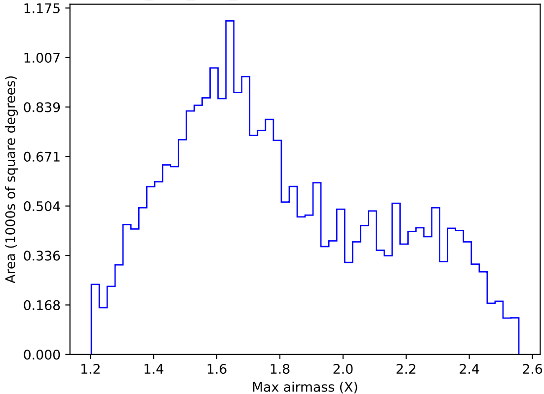
all_long_v3.4_10yrs Yr 1 r band: Max airmass
