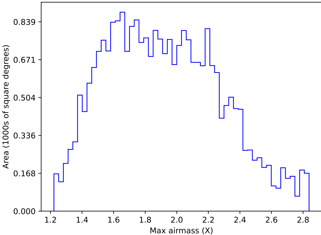
all_long_v3.4_10yrs Yr 1 i band: Max airmass
