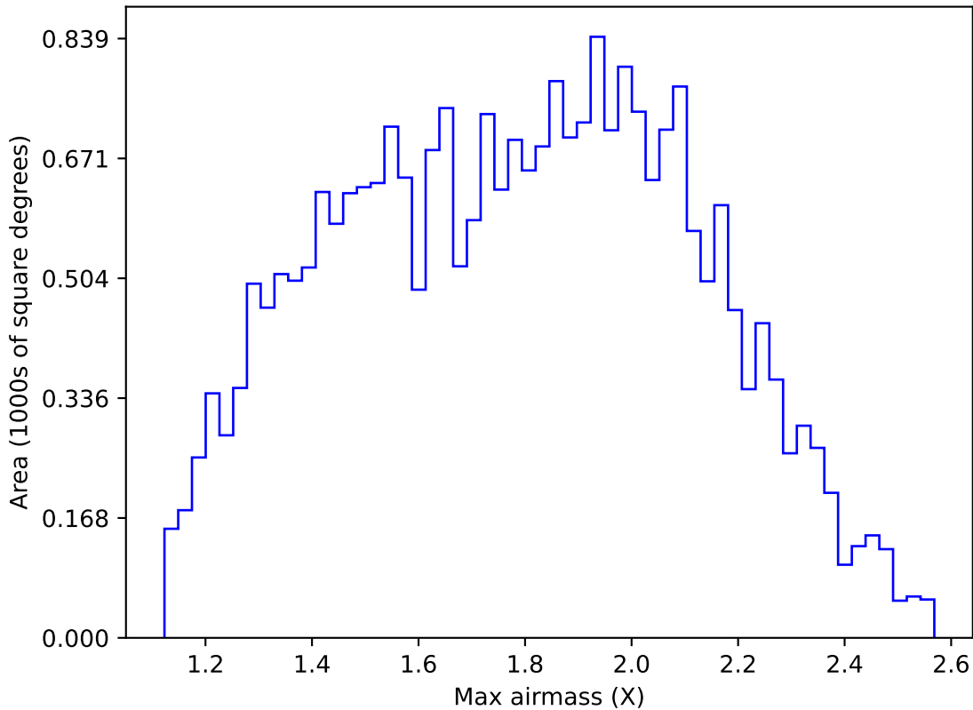
all_long_v3.4_10yrs Yr 1 g band: Max airmass
