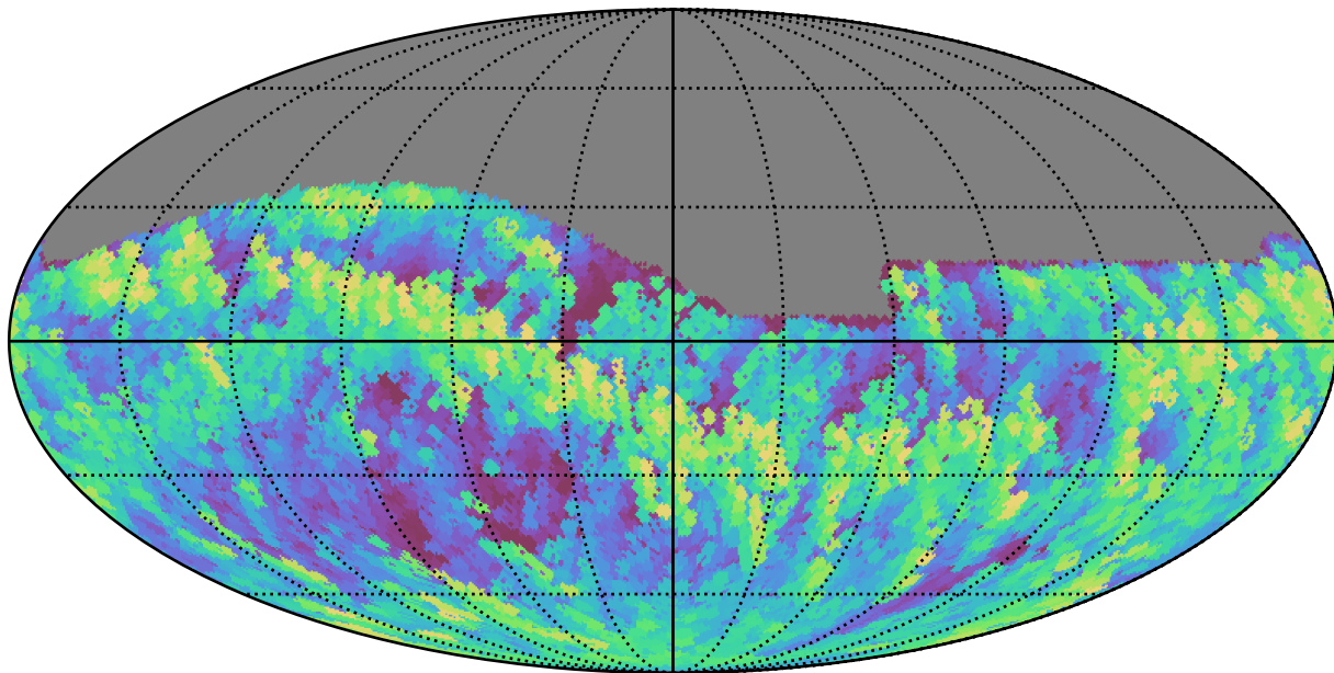
all_long_v3.4_10yrs Yr 1 all bands: Max airmass
