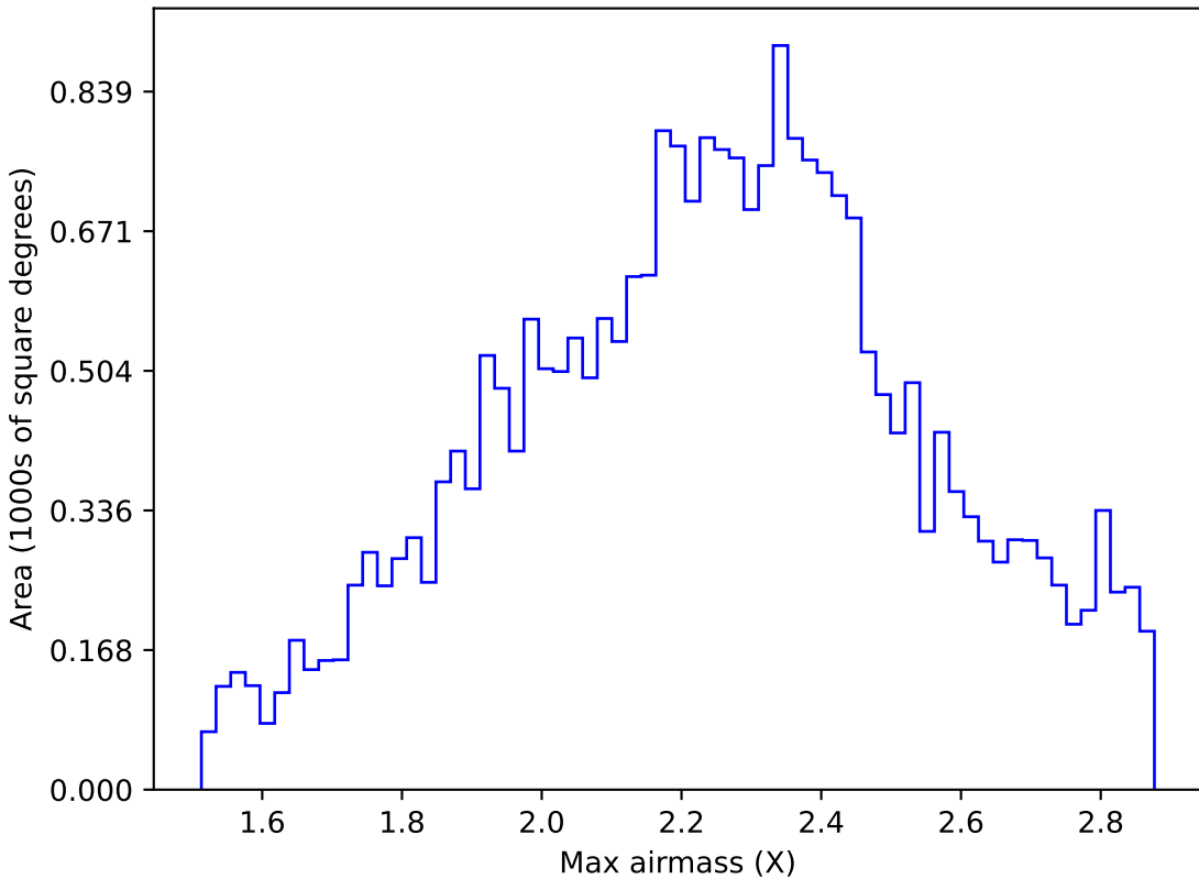
all_long_v3.4_10yrs Yr 1 all bands: Max airmass
