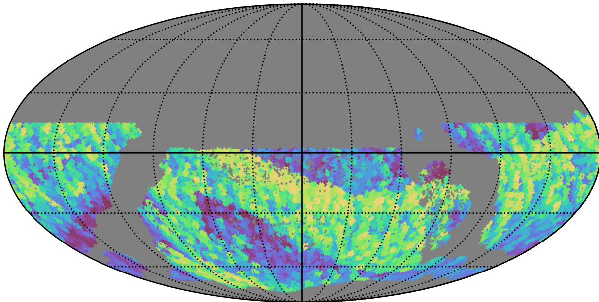
all_long_v3.4_10yrs WFD z band: Max airmass
