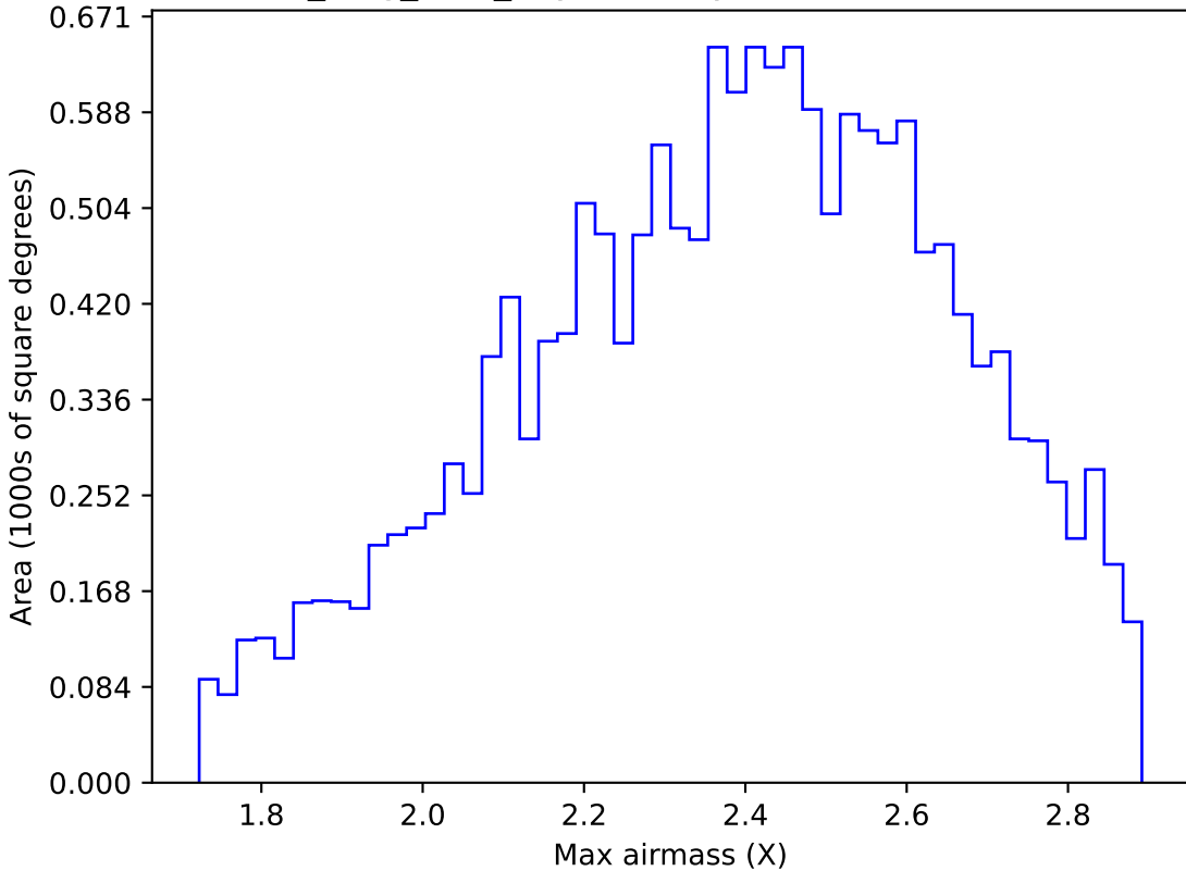
all_long_v3.4_10yrs WFD y band: Max airmass
