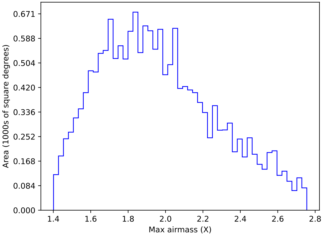
all_long_v3.4_10yrs WFD u band: Max airmass
