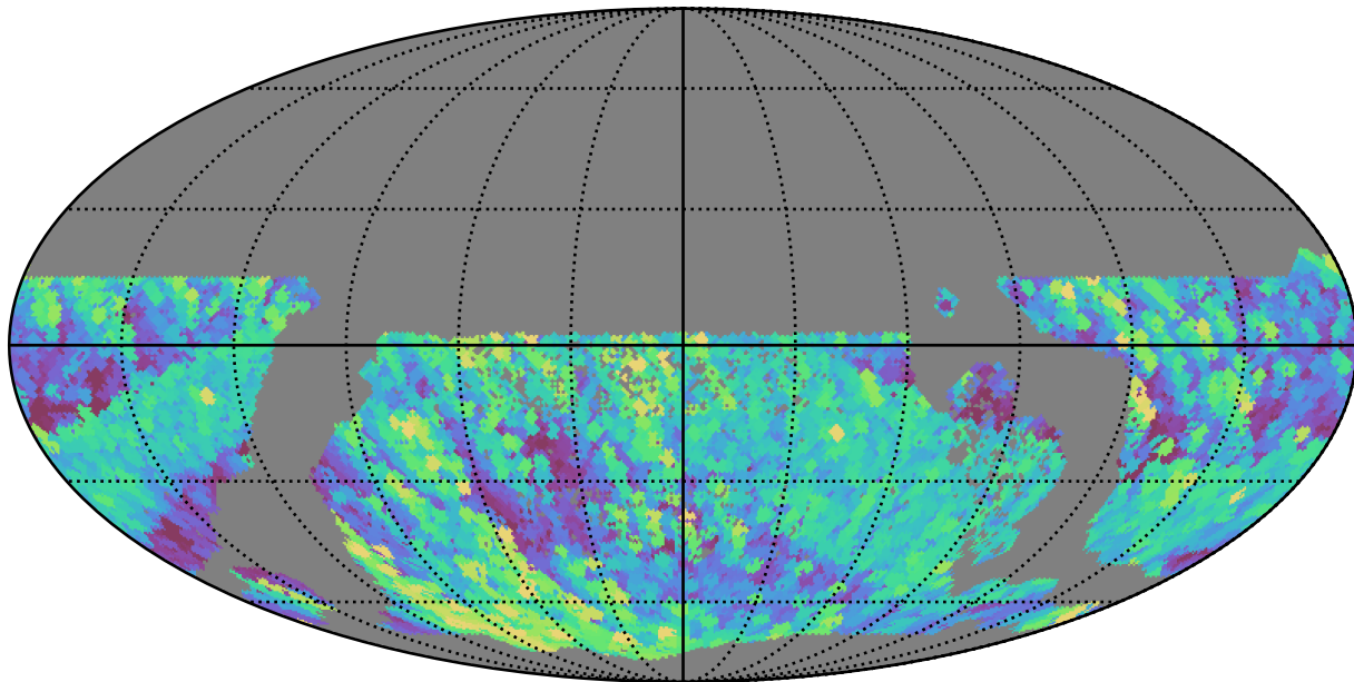
all_long_v3.4_10yrs WFD r band: Max airmass
