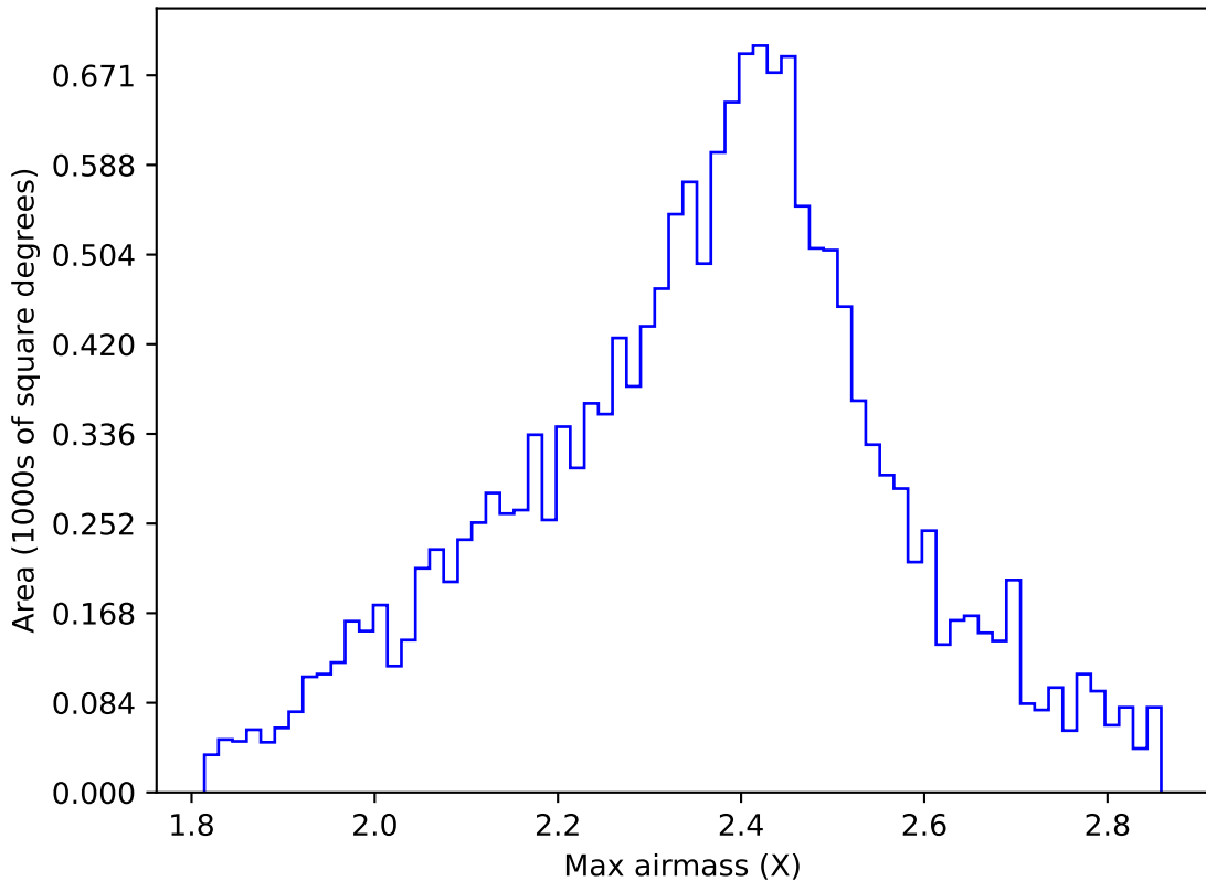
all_long_v3.4_10yrs WFD r band: Max airmass
