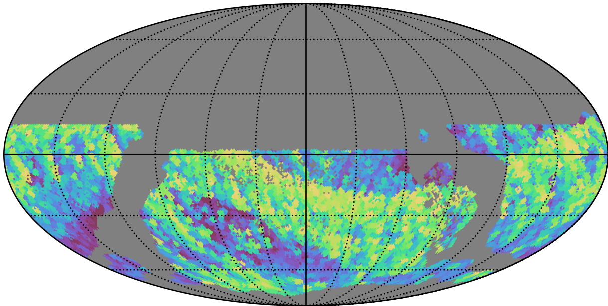
all_long_v3.4_10yrs WFD i band: Max airmass
