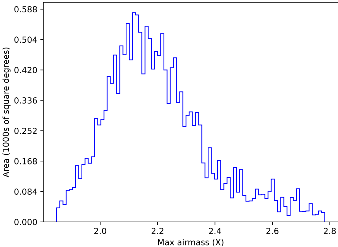
all_long_v3.4_10yrs WFD g band: Max airmass
