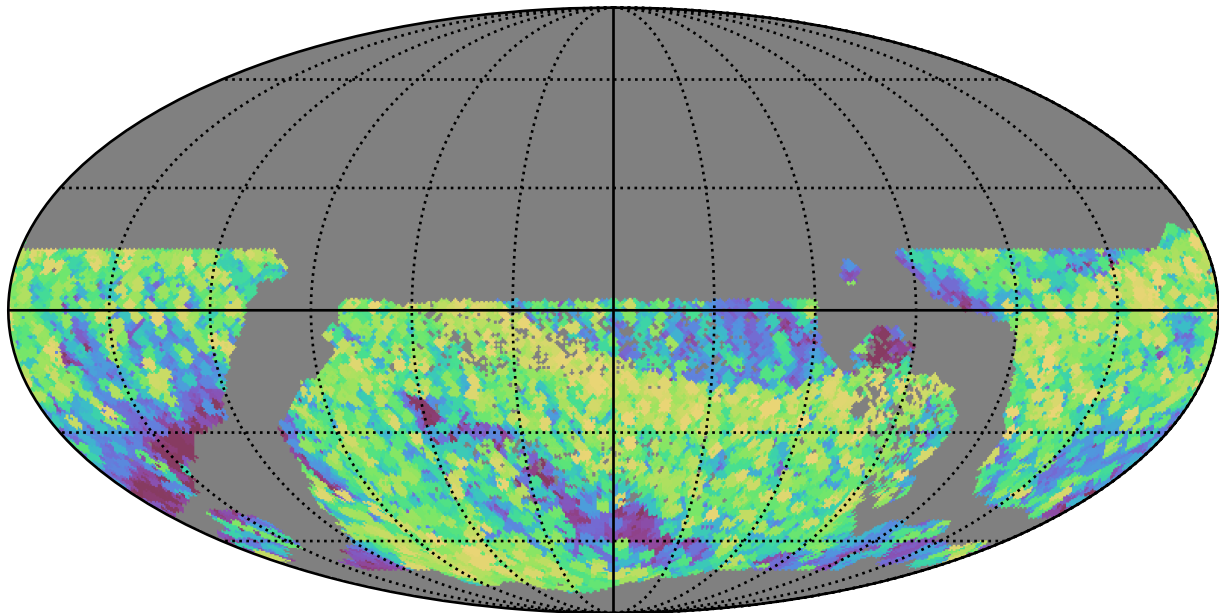
all_long_v3.4_10yrs WFD all bands: Max airmass
