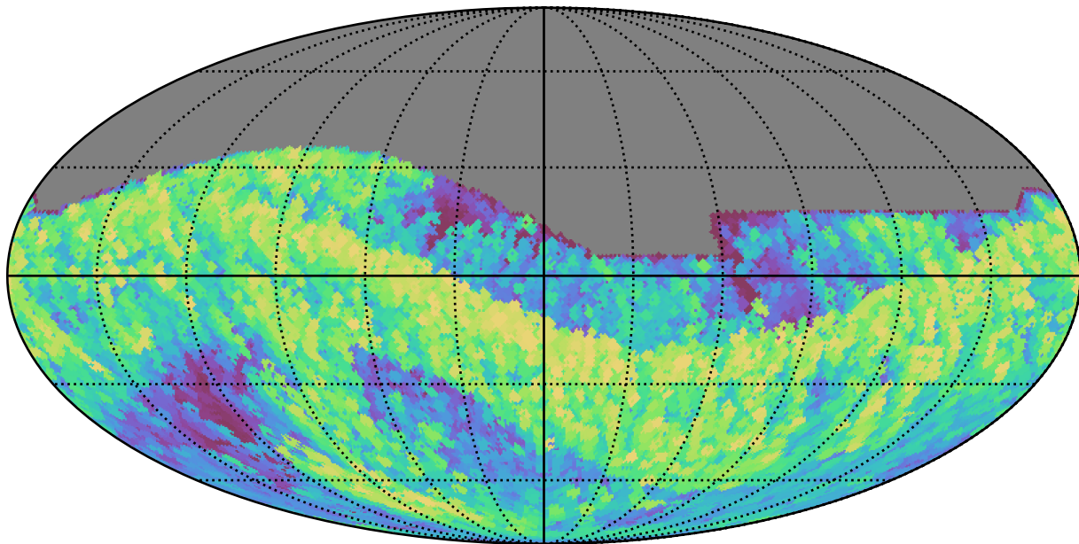
all_long_v3.4_10yrs All sky z band: Max airmass
