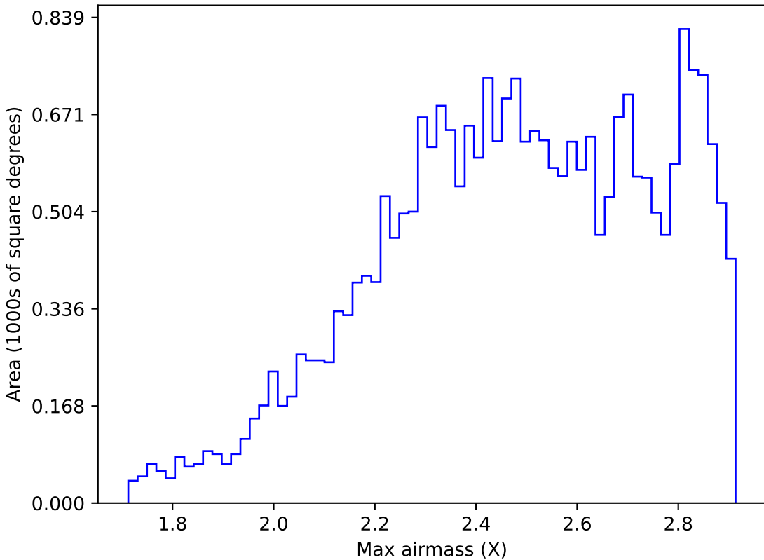
all_long_v3.4_10yrs All sky z band: Max airmass
