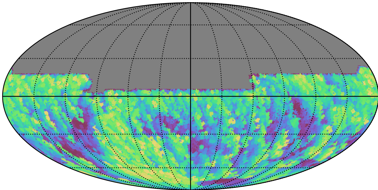
all_long_v3.4_10yrs All sky y band: Max airmass
