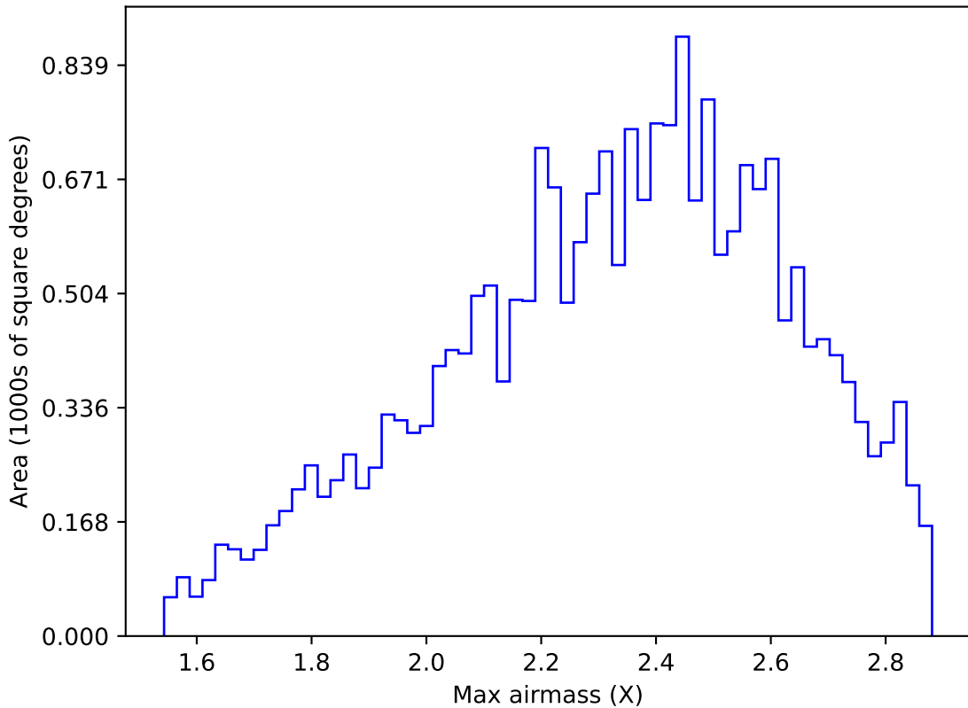
all_long_v3.4_10yrs All sky y band: Max airmass
