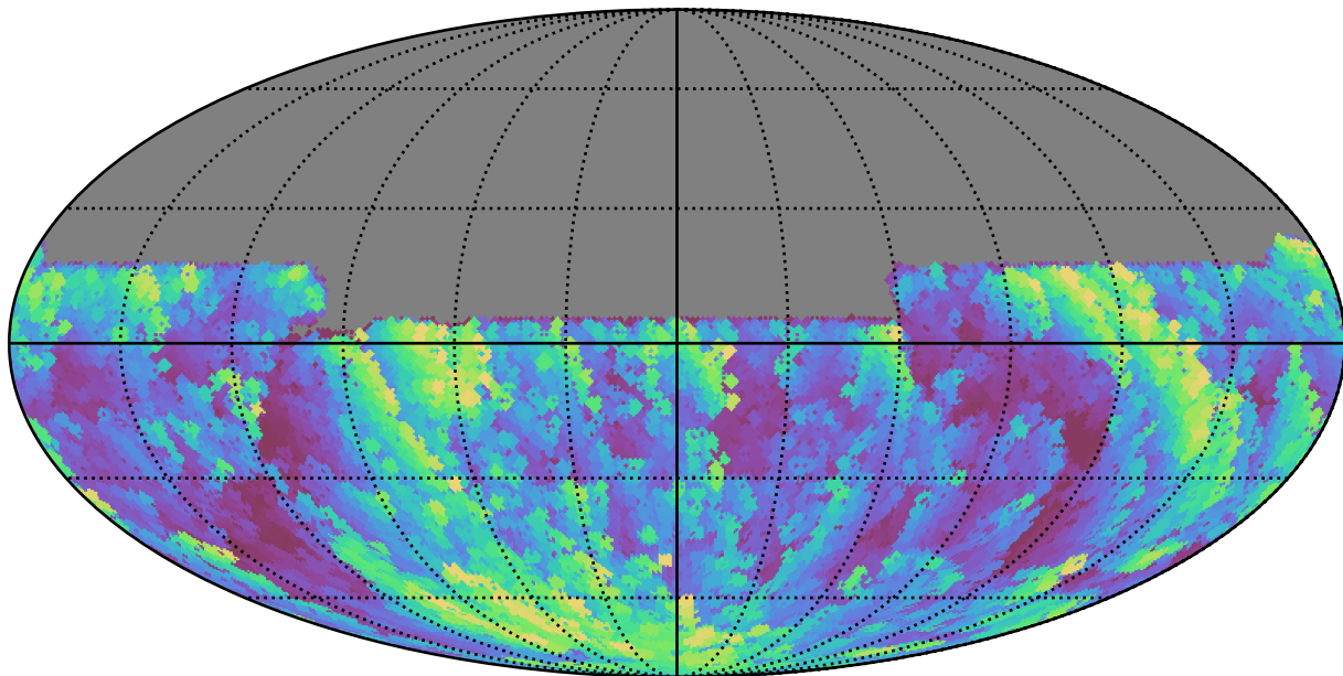
all_long_v3.4_10yrs All sky u band: Max airmass
