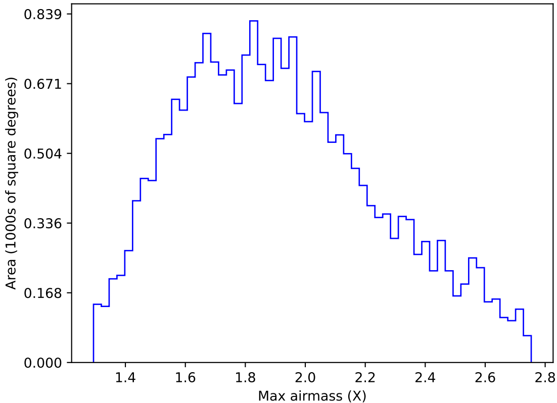
all_long_v3.4_10yrs All sky u band: Max airmass
