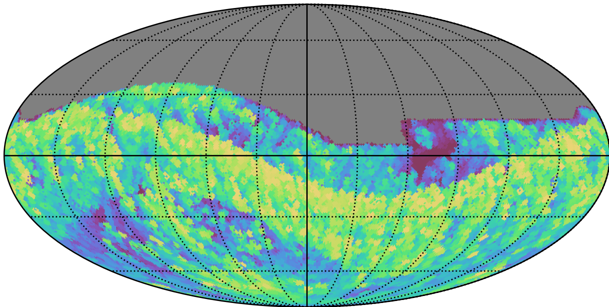
all_long_v3.4_10yrs All sky i band: Max airmass
