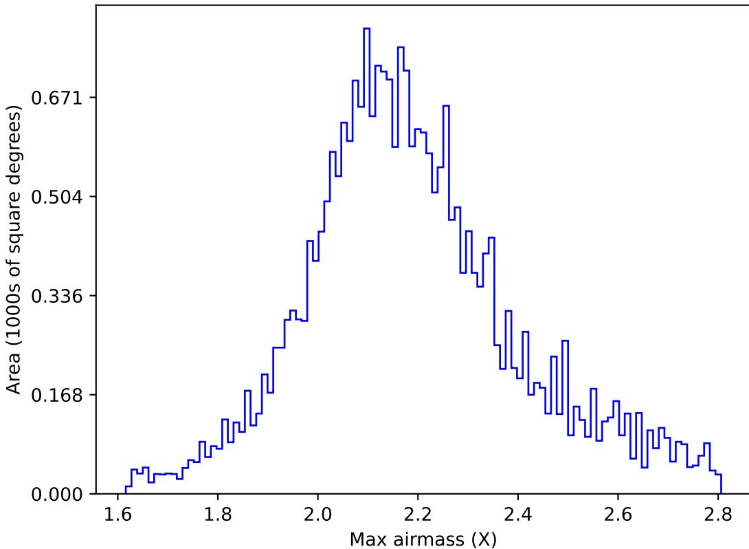
all_long_v3.4_10yrs All sky g band: Max airmass
