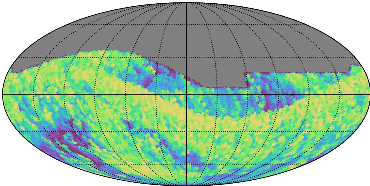
all_long_v3.4_10yrs All sky all bands: Max airmass
