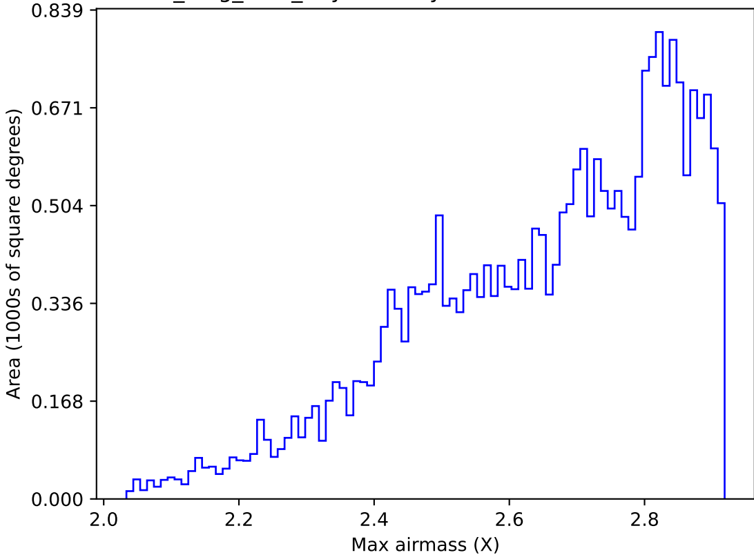
all_long_v3.4_10yrs All sky all bands: Max airmass
