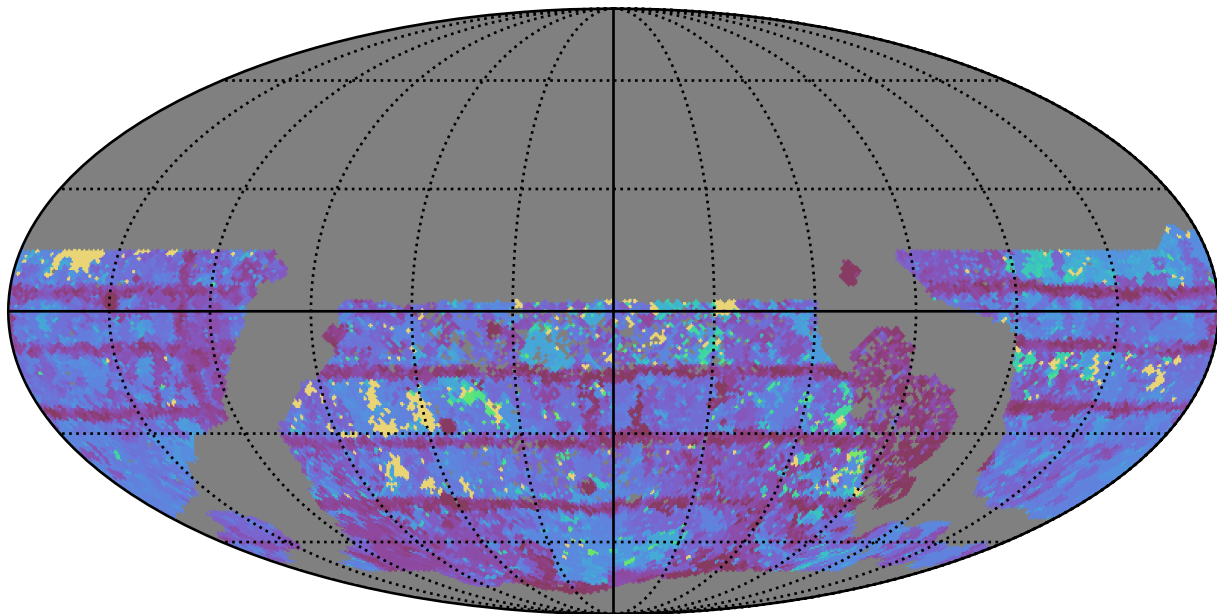
all_long_v3.4_10yrs WFD z band: Max Inter-Night Gap
