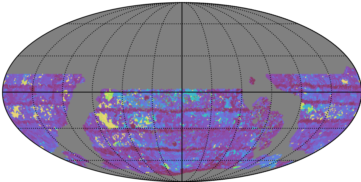
all_long_v3.4_10yrs WFD y band: Max Inter-Night Gap
