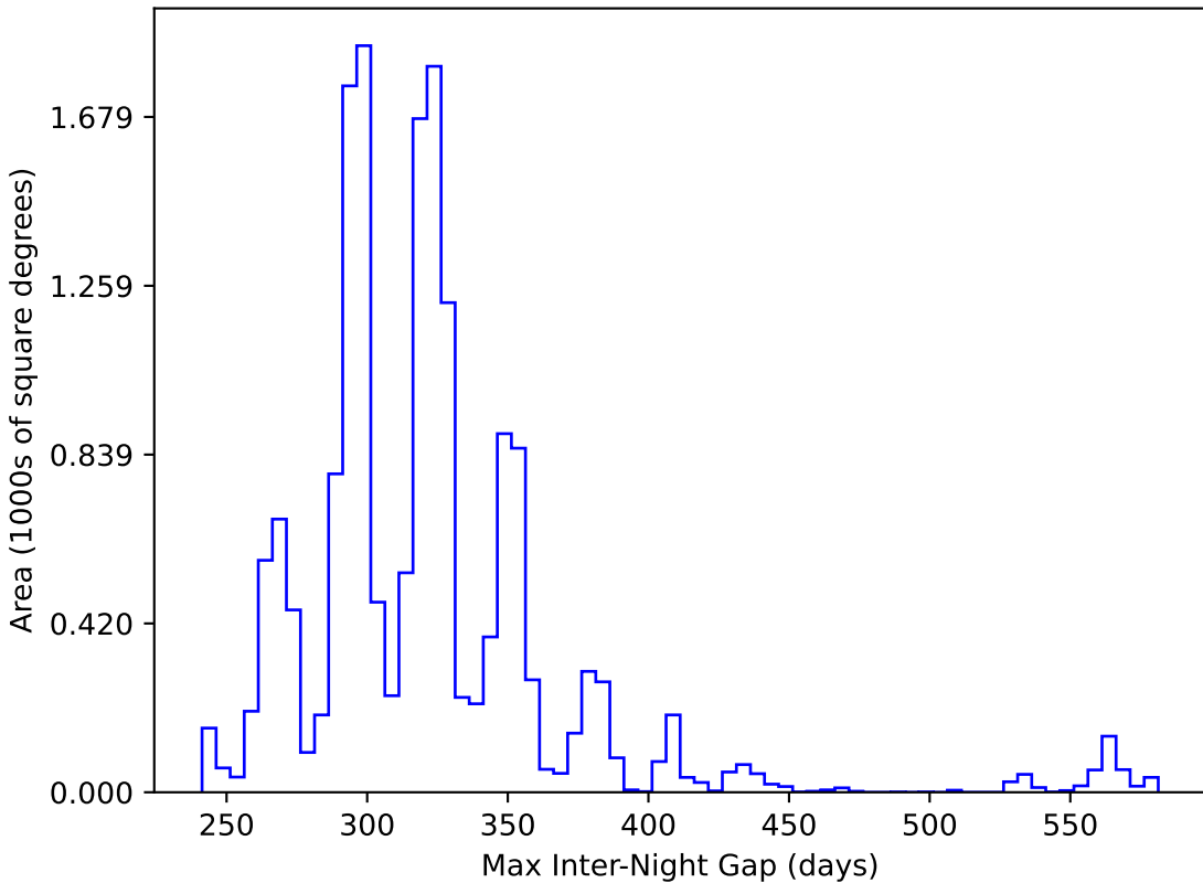
all_long_v3.4_10yrs WFD y band: Max Inter-Night Gap
