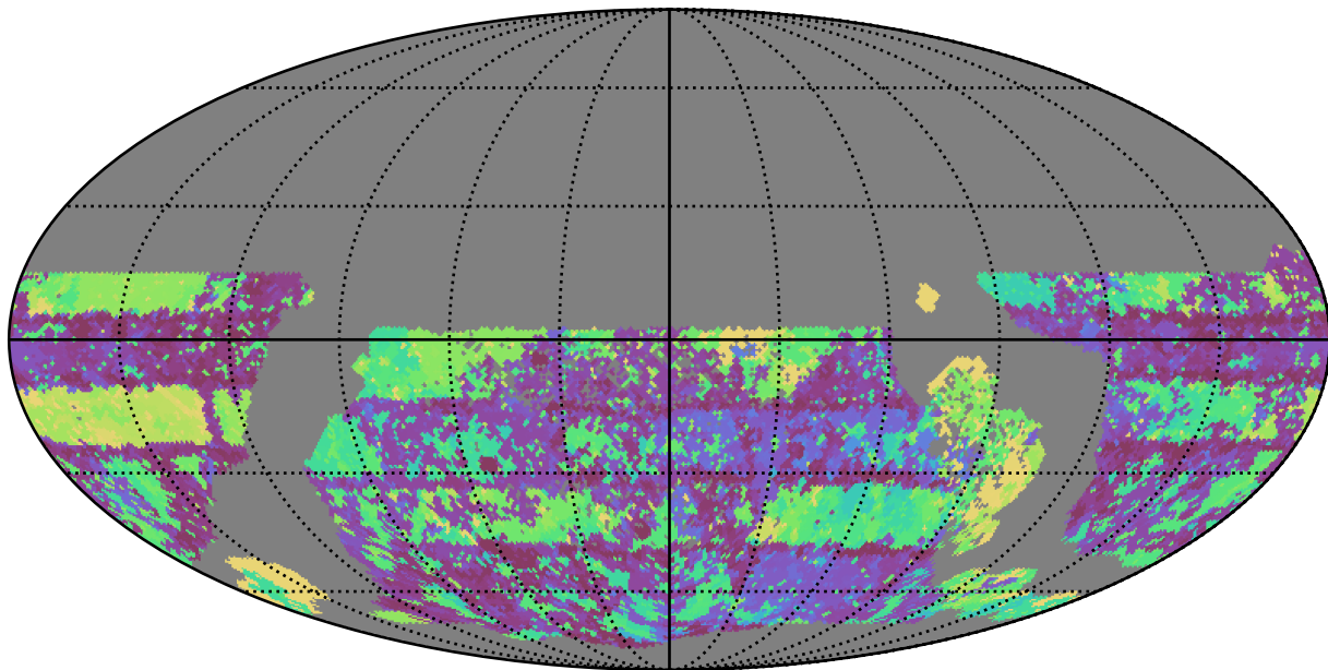
all_long_v3.4_10yrs WFD u band: Max Inter-Night Gap
