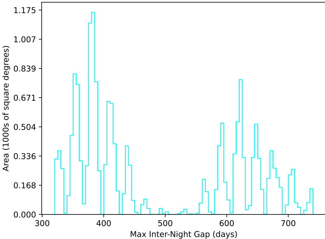
all_long_v3.4_10yrs WFD u band: Max Inter-Night Gap
