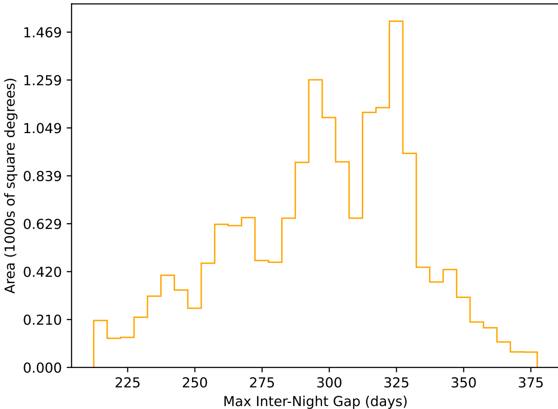
all_long_v3.4_10yrs WFD r band: Max Inter-Night Gap
