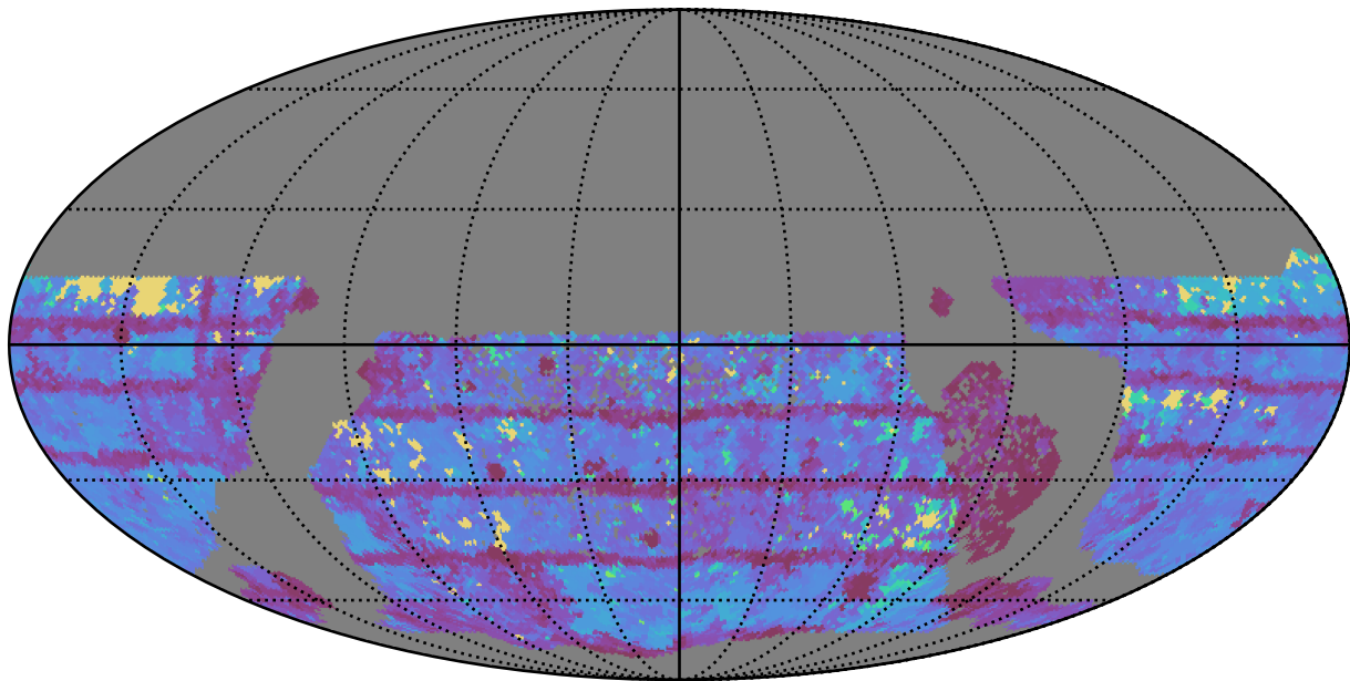
all_long_v3.4_10yrs WFD i band: Max Inter-Night Gap
