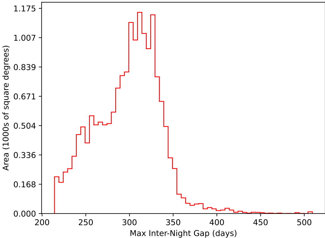
all_long_v3.4_10yrs WFD i band: Max Inter-Night Gap
