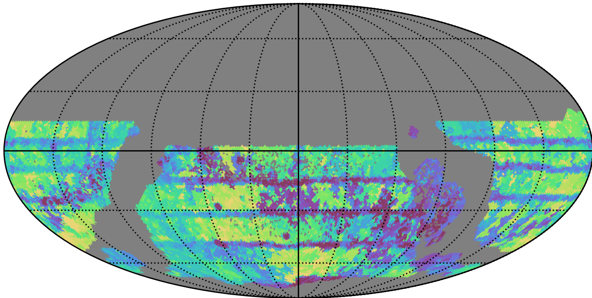
all_long_v3.4_10yrs WFD all bands: Max Inter-Night Gap
