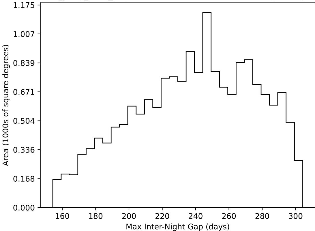
all_long_v3.4_10yrs WFD all bands: Max Inter-Night Gap
