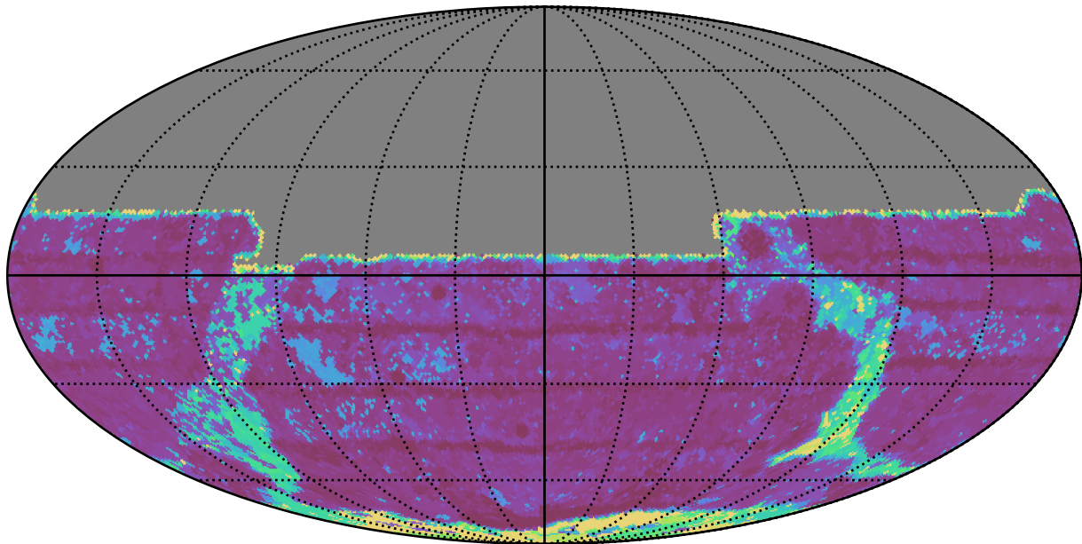
all_long_v3.4_10yrs All sky y band: Max Inter-Night Gap
