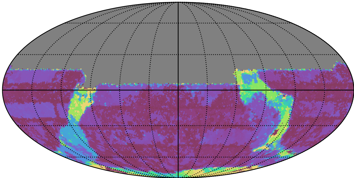
all_long_v3.4_10yrs All sky u band: Max Inter-Night Gap
