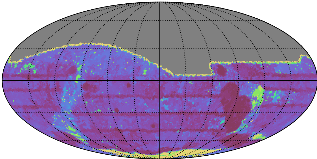
all_long_v3.4_10yrs All sky r band: Max Inter-Night Gap
