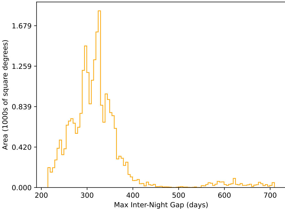
all_long_v3.4_10yrs All sky r band: Max Inter-Night Gap
