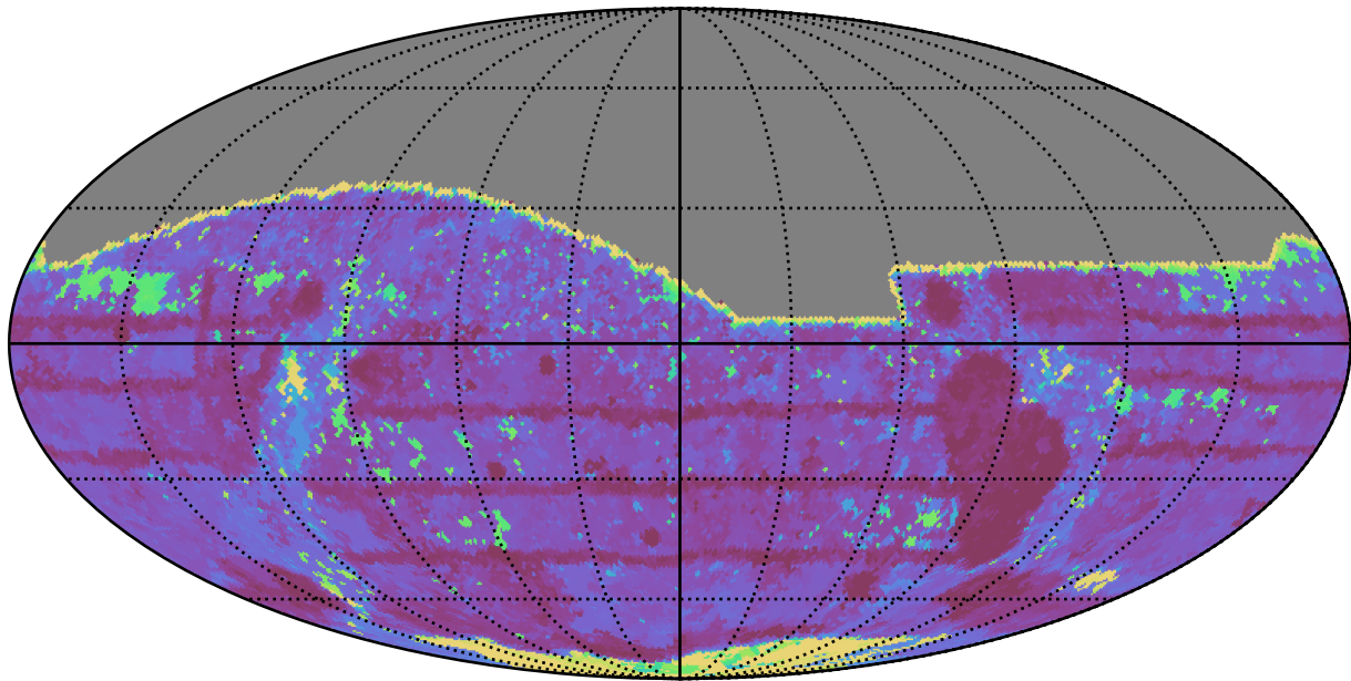
all_long_v3.4_10yrs All sky i band: Max Inter-Night Gap
