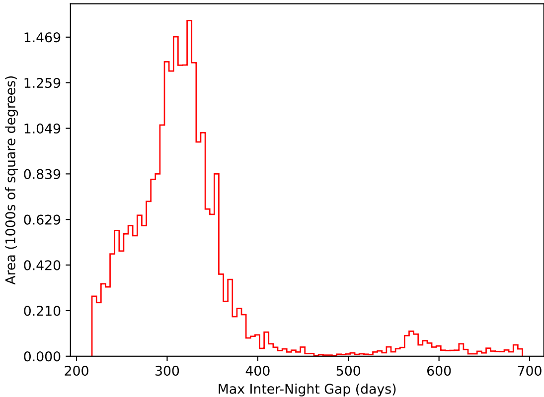
all_long_v3.4_10yrs All sky i band: Max Inter-Night Gap
