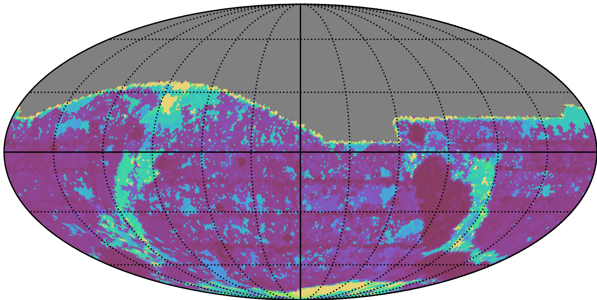
all_long_v3.4_10yrs All sky g band: Max Inter-Night Gap
