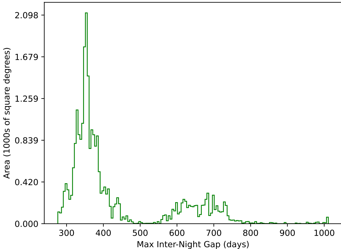
all_long_v3.4_10yrs All sky g band: Max Inter-Night Gap
