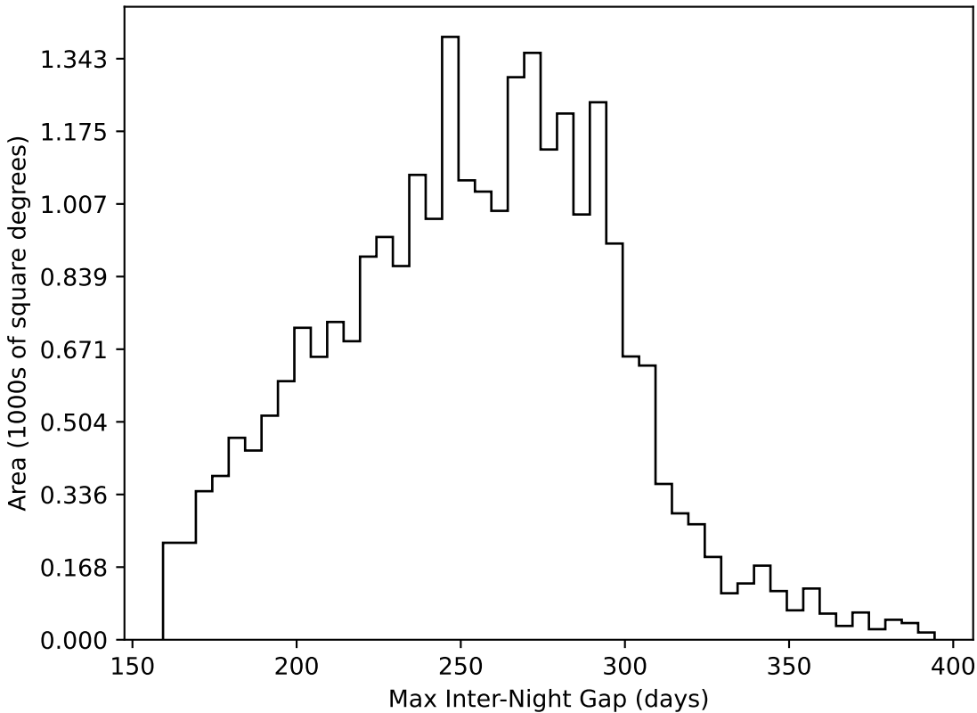
all_long_v3.4_10yrs All sky all bands: Max Inter-Night Gap
