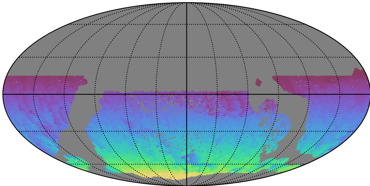
all_long_v3.4_10yrs WFD all bands: Max HA
