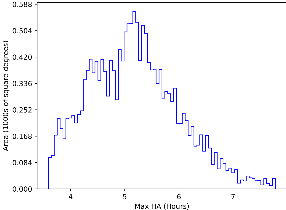
all_long_v3.4_10yrs WFD all bands: Max HA
