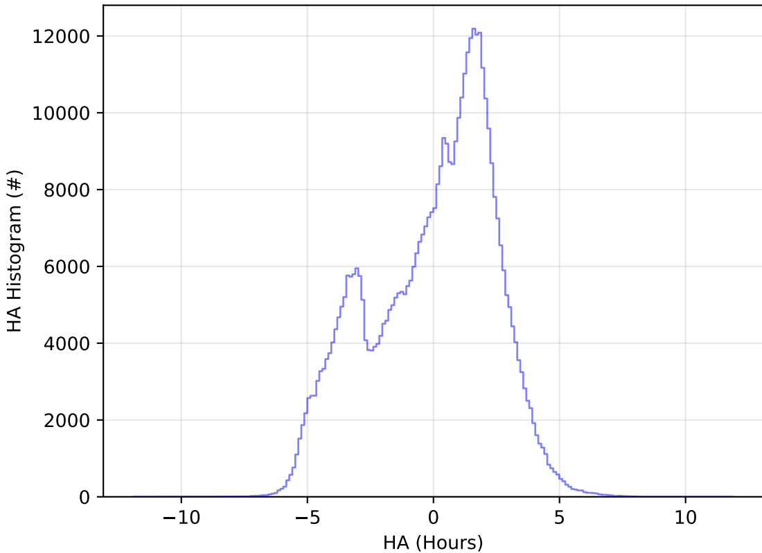
all_long_v3.4_10yrs WFD r band: HA Histogram
