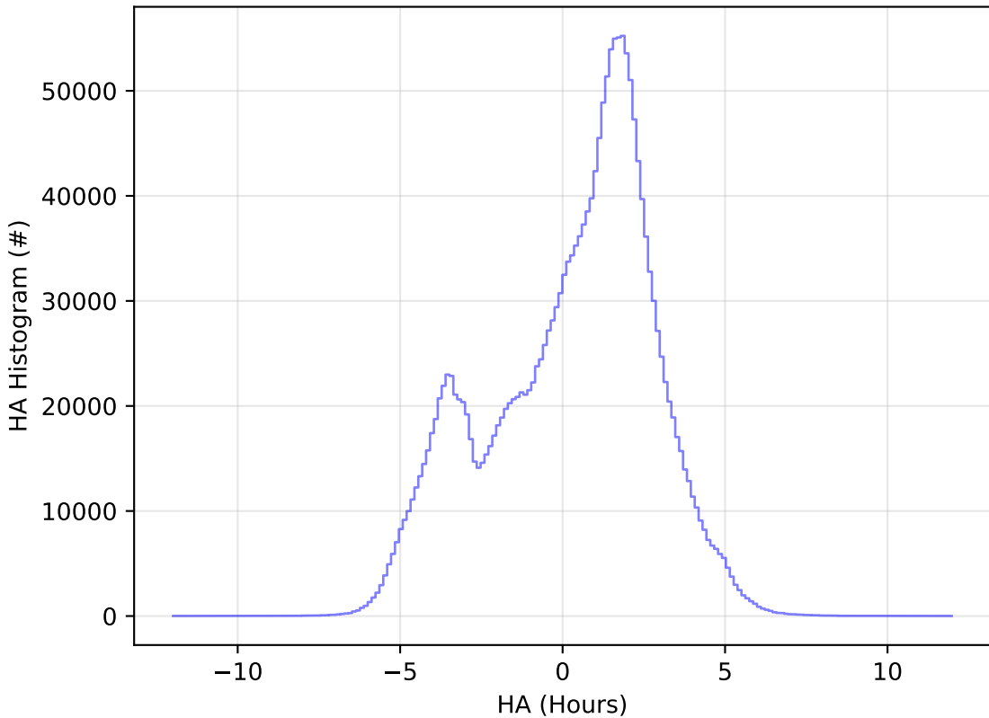
all_long_v3.4_10yrs All sky all bands: HA Histogram
