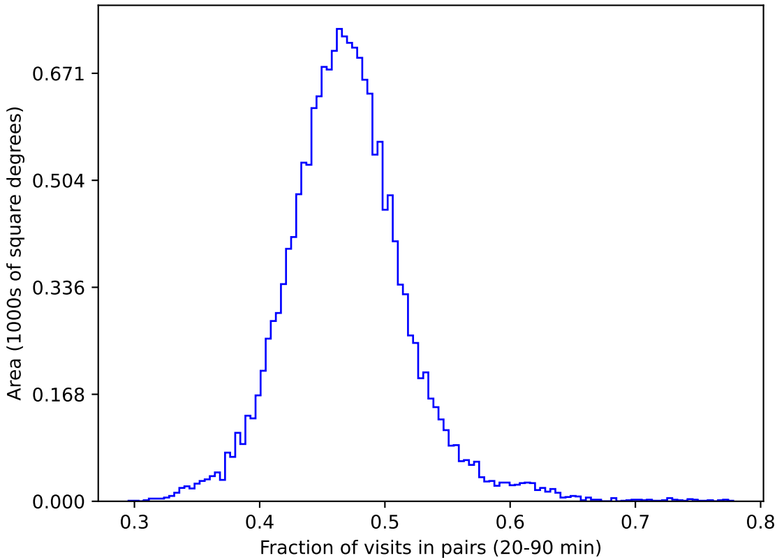
all_long_v3.4_10yrs gri WFD: Fraction of visits in pairs (20-90 min)
