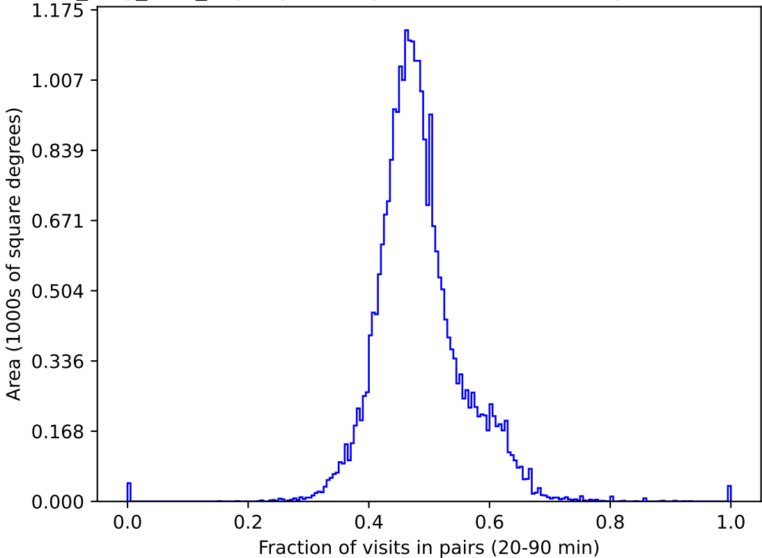
all_long_v3.4_10yrs gri All sky: Fraction of visits in pairs (20-90 min)
